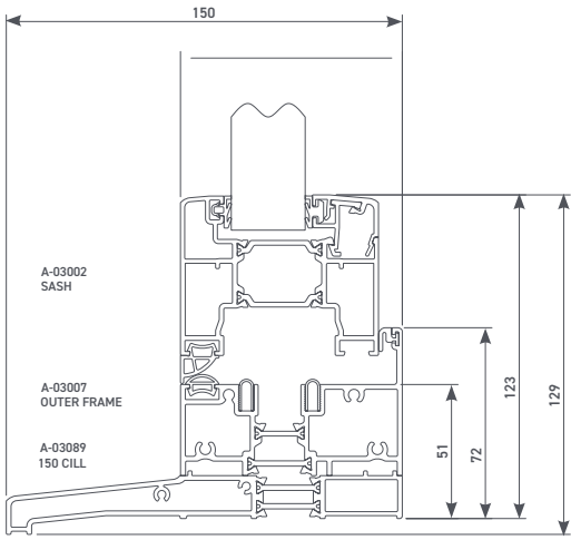
150mm cill with outer frame & sash profile
