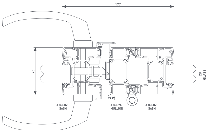
Traffic door connecting to sliding mullion
